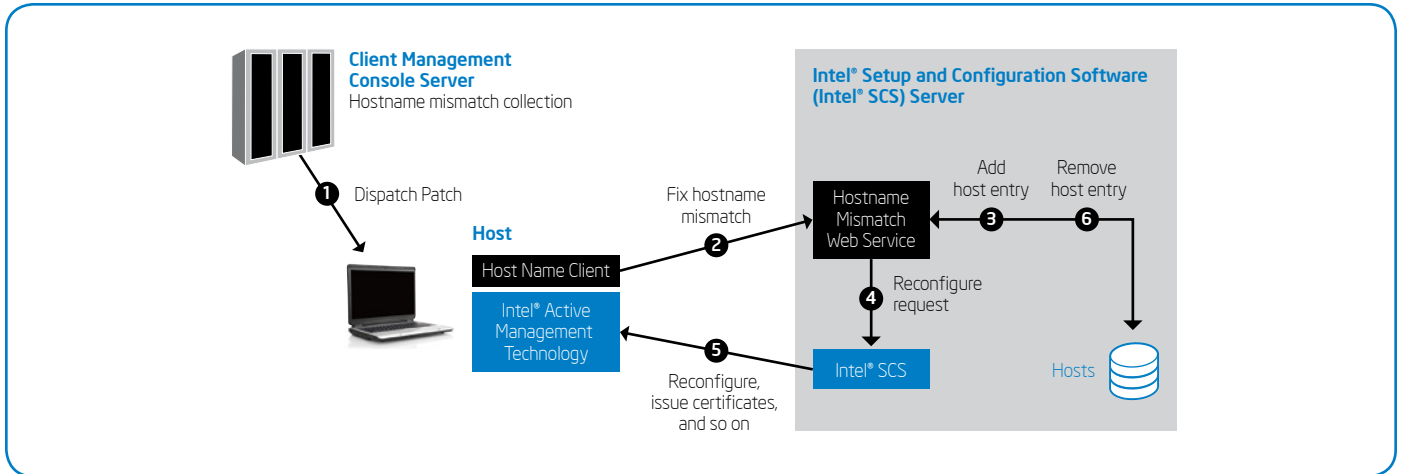
Figure 5. To resolve the issue of hostname mismatches, we wrote code that adds an entry to the host’s file on the server that runs Intel® Setup and Configuration Software (Intel® SCS) and then lets Intel SCS perform its task.
