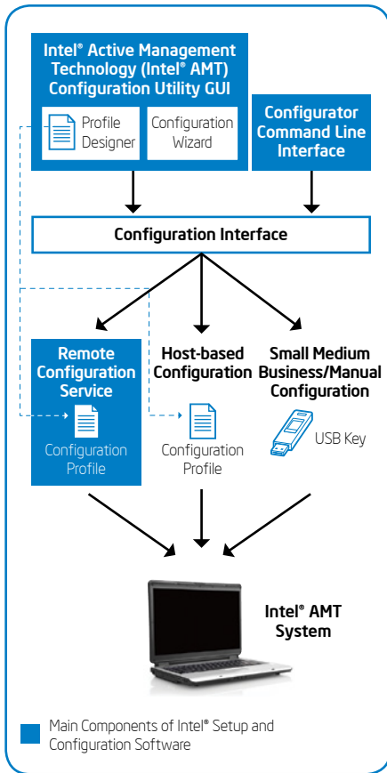
Figure 1. Main components of Intel® Setup and Configuration Software 7.0 and methods for configuring clients based on Intel® Active Management Technology.
