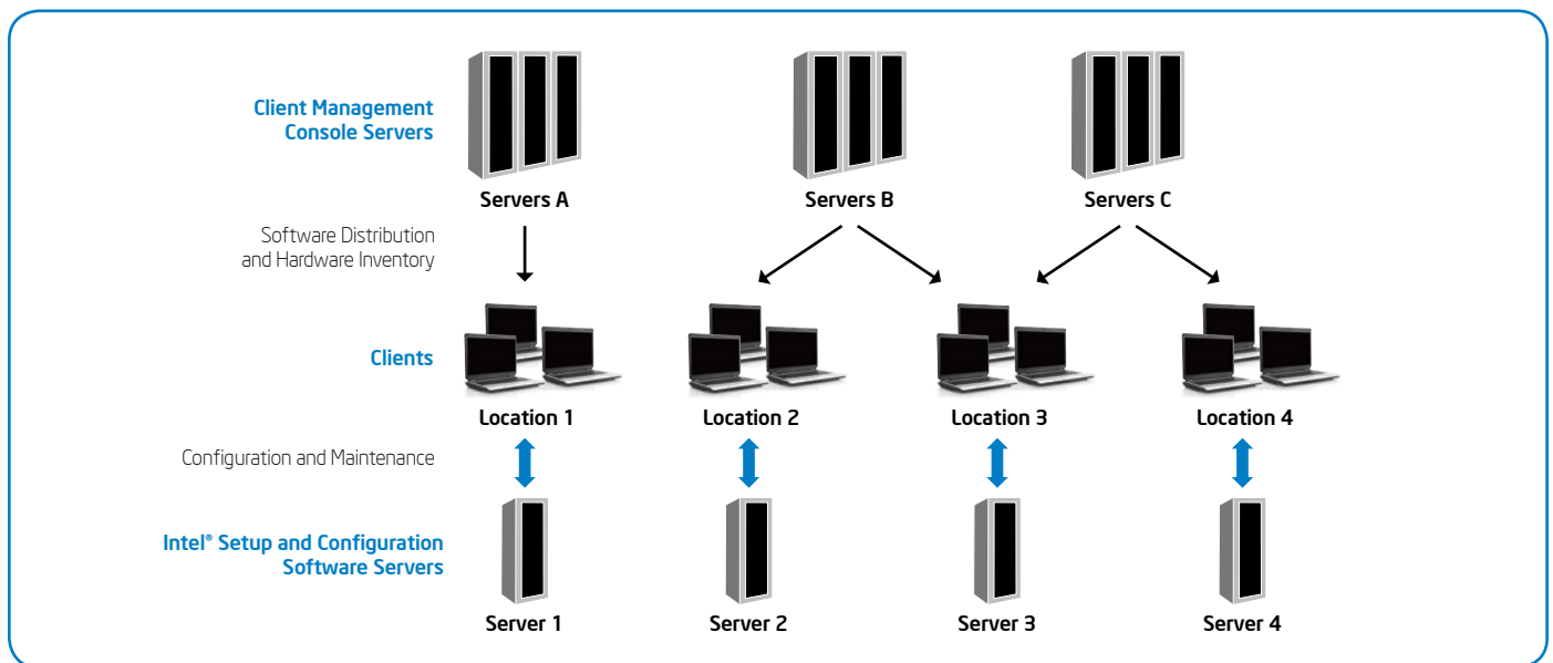
Figure 3. Our new client management solution uses the client management console for software distribution, inventory, and database functions, and uses Intel® Setup and Configuration Software for Intel® Active Management Technology configuration and maintenance.
