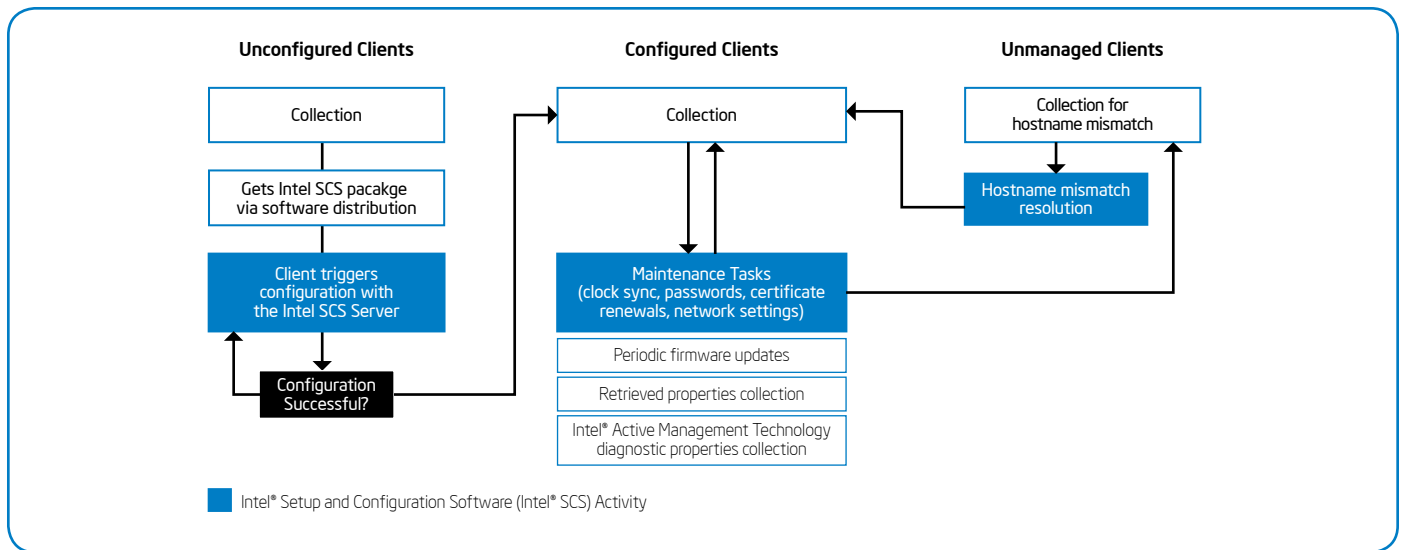
Figure 4. This diagram shows the Intel® Active Management Technology flow for unconfigured, configured, and unmanaged clients.
