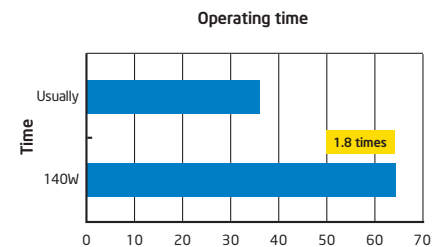
Figure 6. Realized operation of 64 hours, which is approximately 1.8 times the time when the standard operation time for the fuel tank is assumed to be 36 hours
